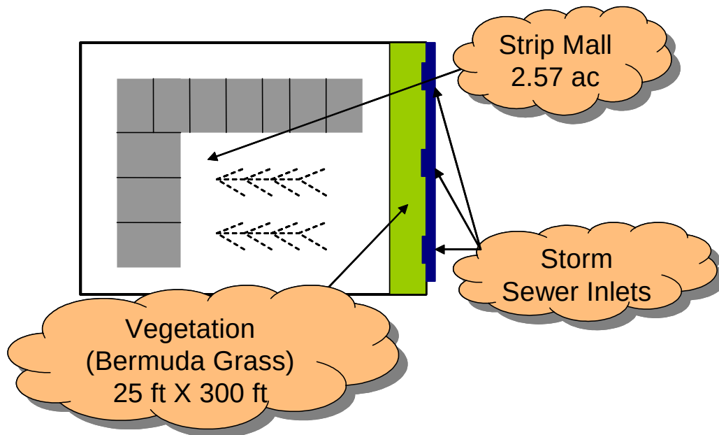
Figure 5-13 Strip Mall Development for Example Problem 5.3
