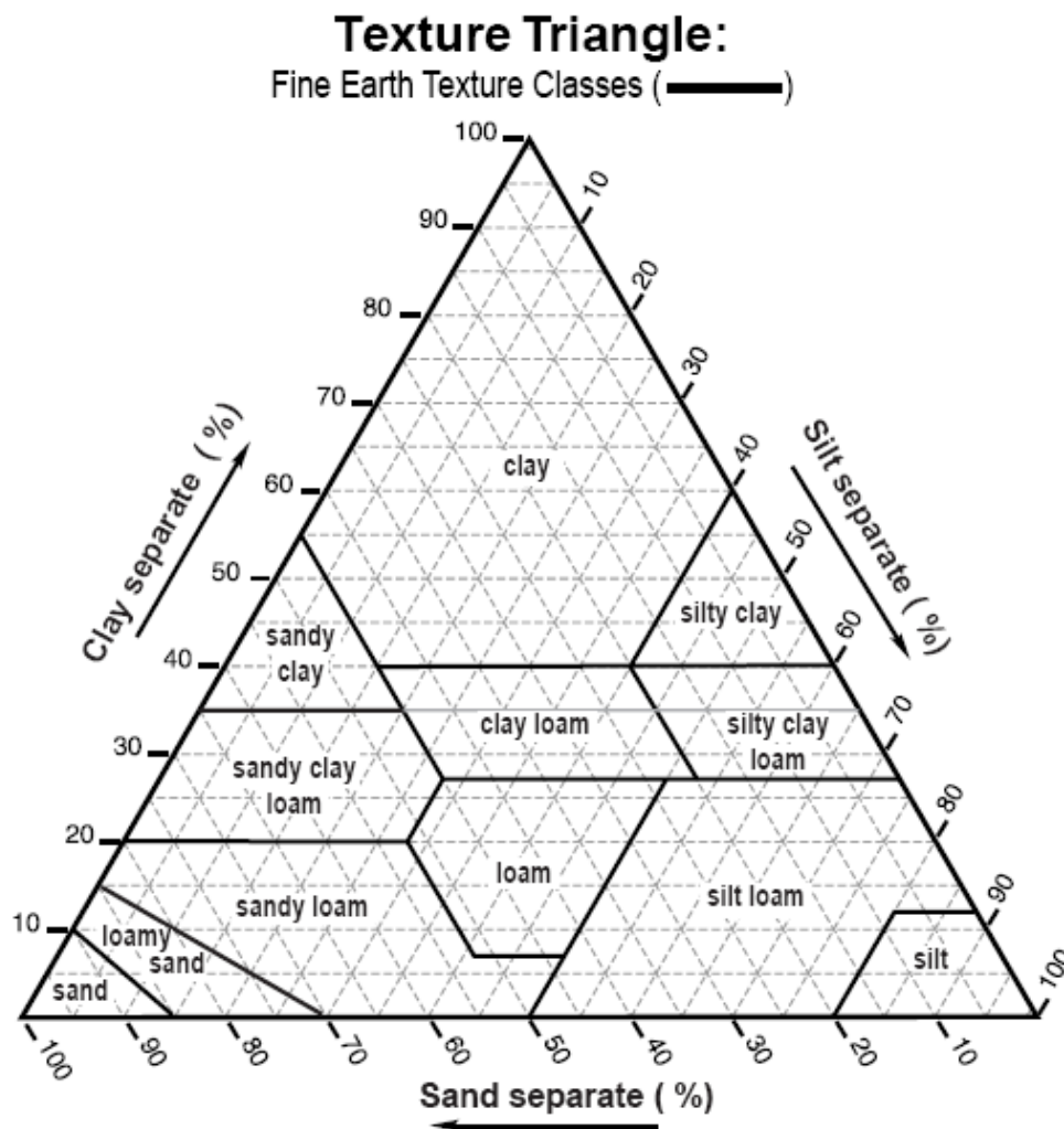
Figure 8.1 USDA Textural Classification Triangle
